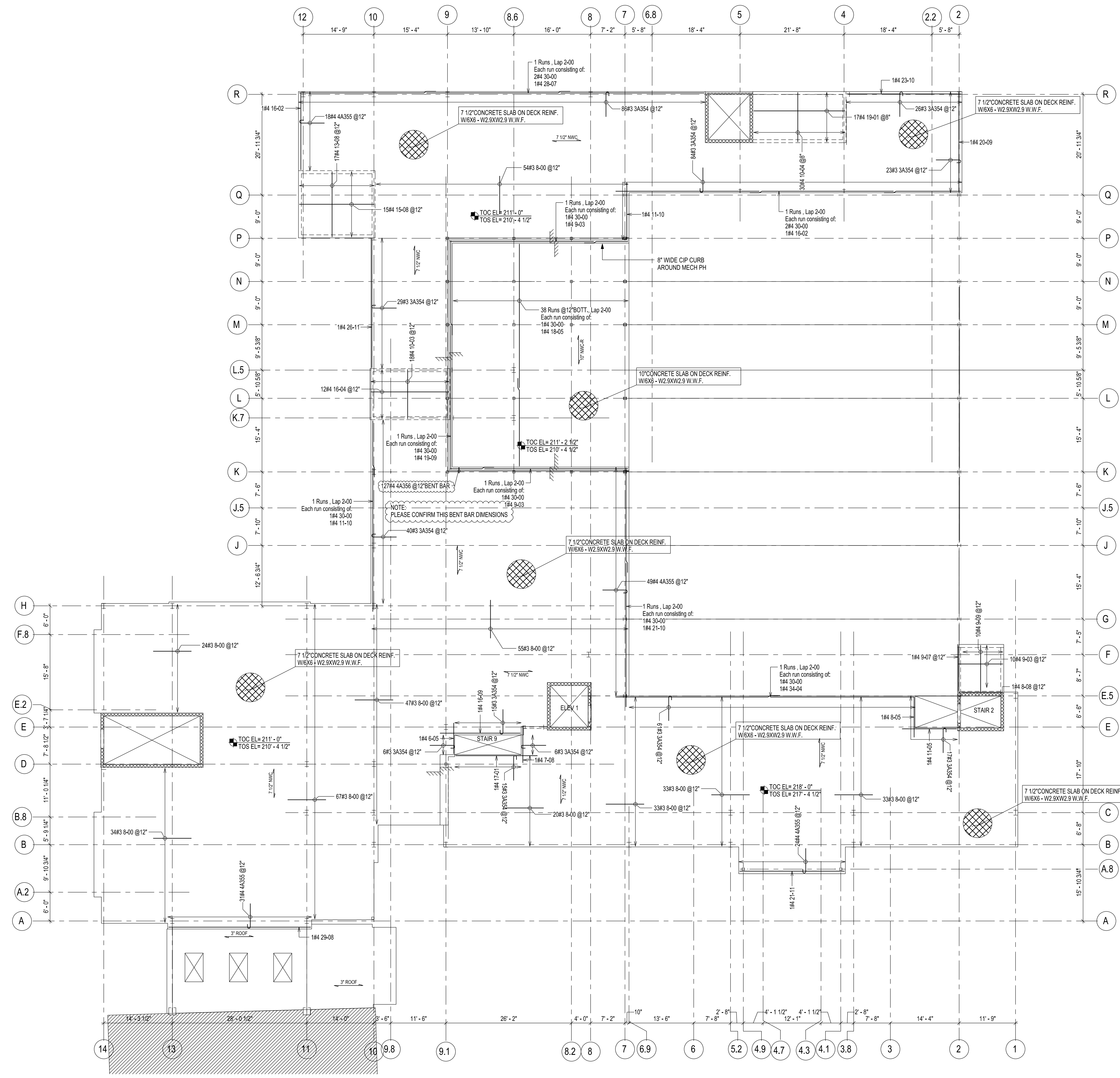
1 SLAB ON DECK PLAN - LEVEL 2 R201
